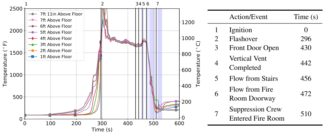
Figure 3.78: Temperatures in fire room (bedroom 2) for Experiment 7. Blue vertical bars indicate time and duration of water flow.
