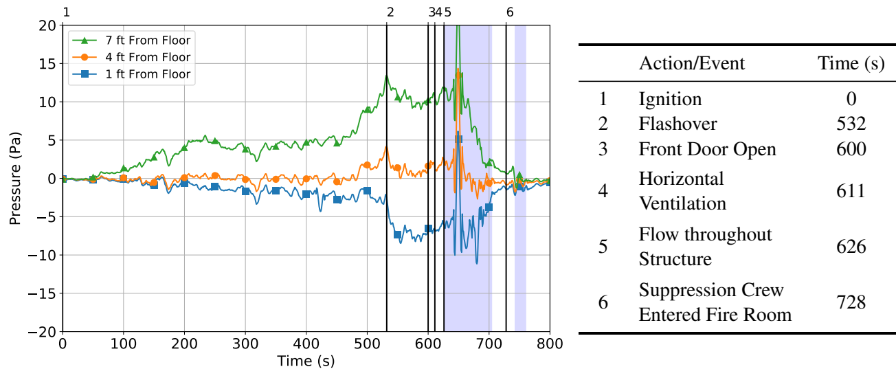
Figure 3.196: Pressures in the fire room (kitchen) for Experiment 16. Blue vertical bars indicate time and duration of water flow.
