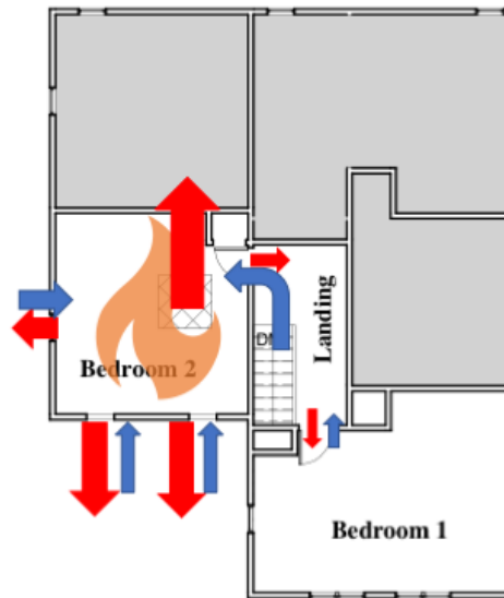
(c) After Vertical Ventilation
