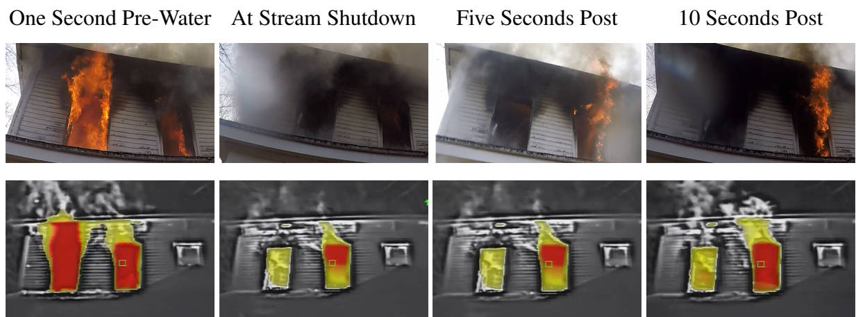
Figure 4.21: Visual representation of the effect of the initial water application on the fire room where the ceiling has failed for Experiment 14. Standard video from firefighters helmet from the A side (top), and infrared video from the A side (bottom). The columns are 1 s prior to water application (left) at the point the stream was shut down (left middle), 5 s post water application (Right Middle), and 10 s post water application (right).
