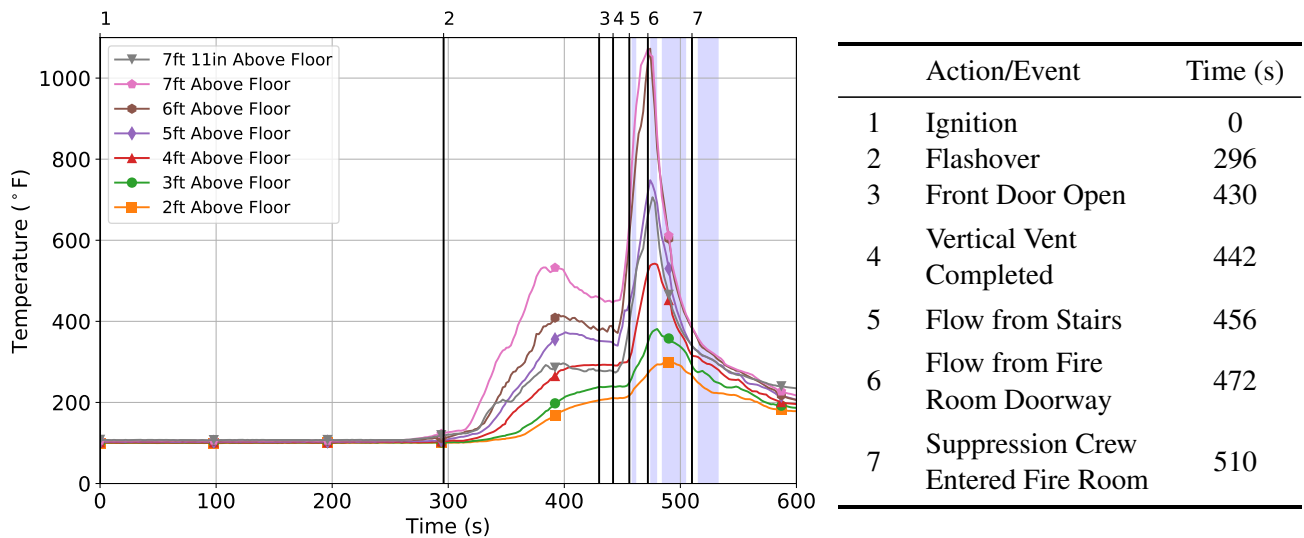
Figure 3.79: Temperatures in attic for Experiment 7. Blue vertical bars indicate time and duration of water flow.
