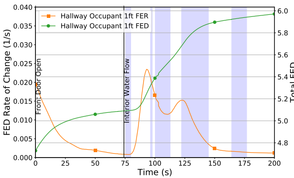
(c) Experiment 13 – Hallway 1 ft FED
