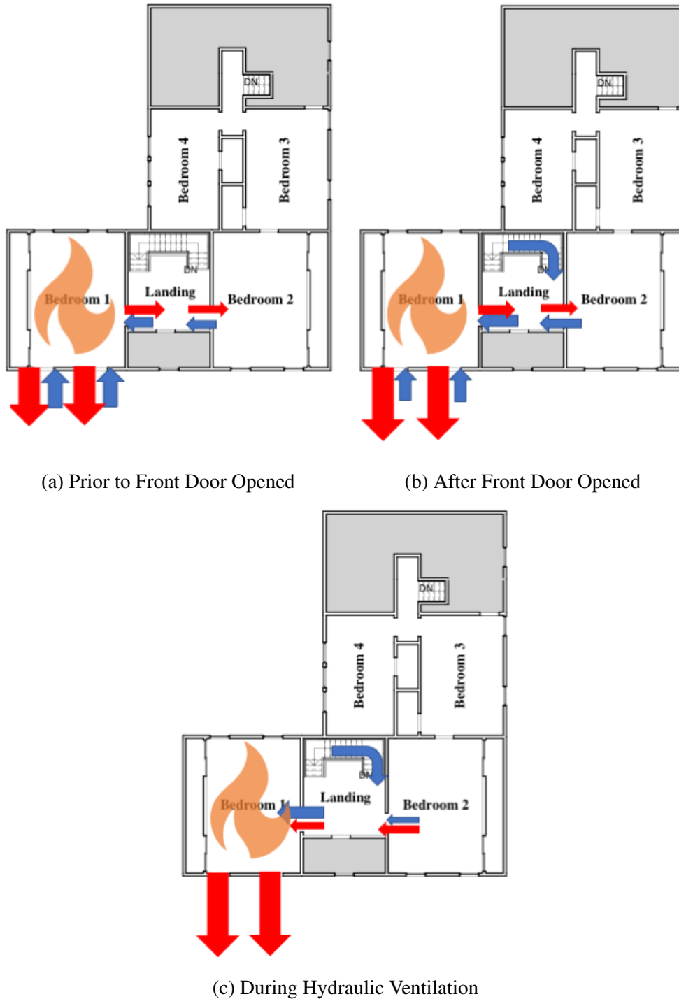
Figure 3.24: Changes in flow during Experiment 2. Red arrows indicate the flow of combustion products, blue arrows indicate the flow of fresh air, and the sizes of the arrows indicate the relative magnitude of the flow through each opening.
