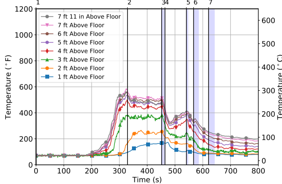
(b) Hallway Temperatures
