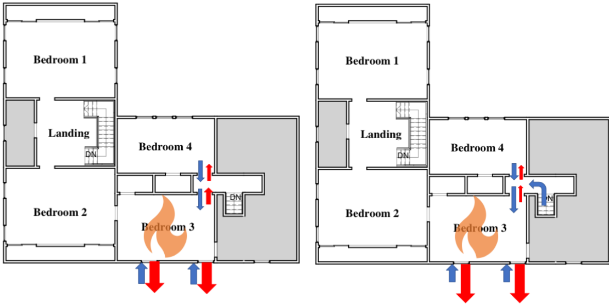
(a) Prior to Front Door Opened
