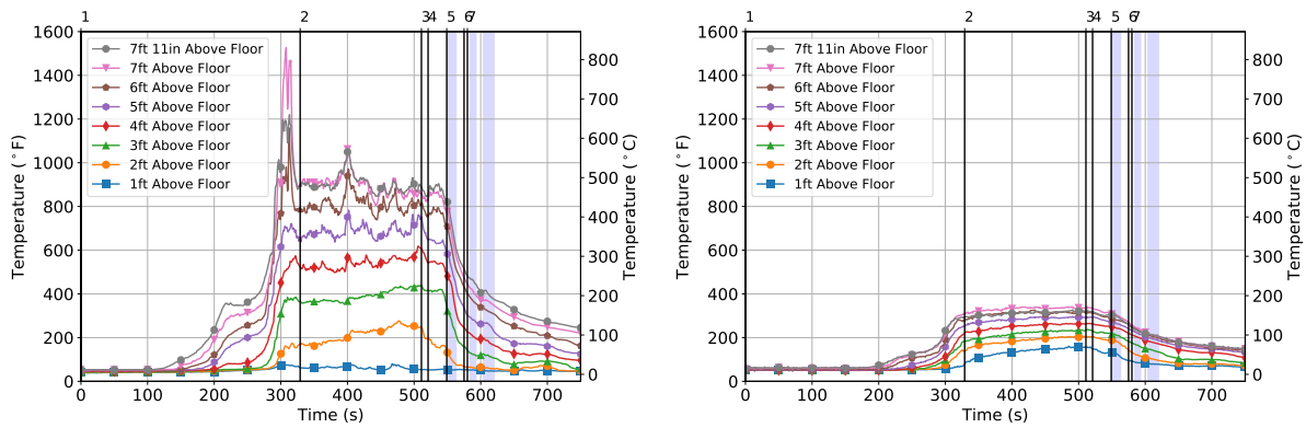
(a) Hallway Temperatures
