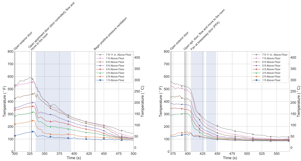
(a) Experiment 2A Living Room Temperatures (b) Experiment 2B Living Room Temperatures
