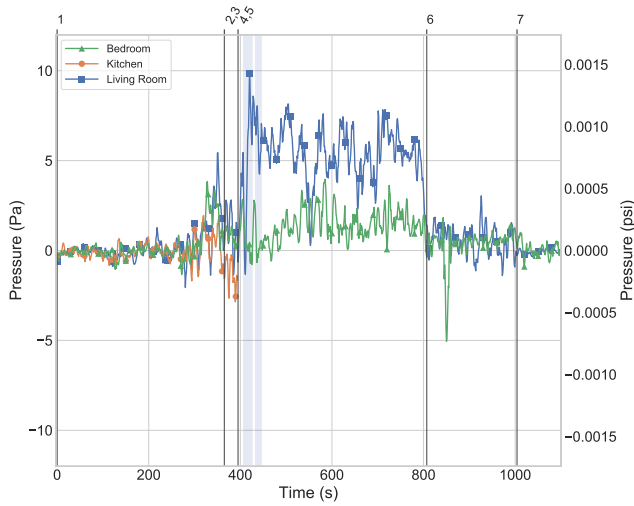
Figure 3.84: Fire apartment pressures for Experiment 2B. Each pressure tap was installed 4 ft above the floor. Blue shaded regions indicate time and duration of water flow.
