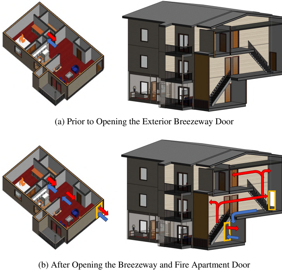
Figure 3.6: Changes in gas flow during Experiment 1A. Red arrows indicate the flow of combustion products, blue arrows indicate the flow of fresh air, and the size of the arrows indicate the relative magnitude of the flow. Yellow boxes indicate ventilation openings.
