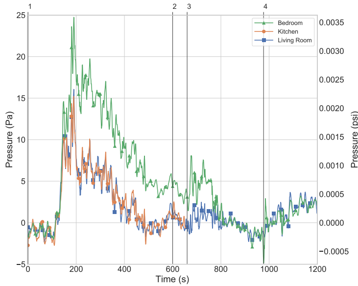
Figure 3.19: Fire apartment pressures for Experiment 1B. Each pressure tap was installed 4 ft above the floor.
