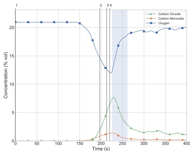
Figure 3.32: Living room gas concentrations for Experiment 1C. Measurement location was 4 ft above the floor. Blue shaded regions indicate time and duration of water flow.
